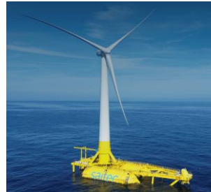
SAITEC's DemoSATH
